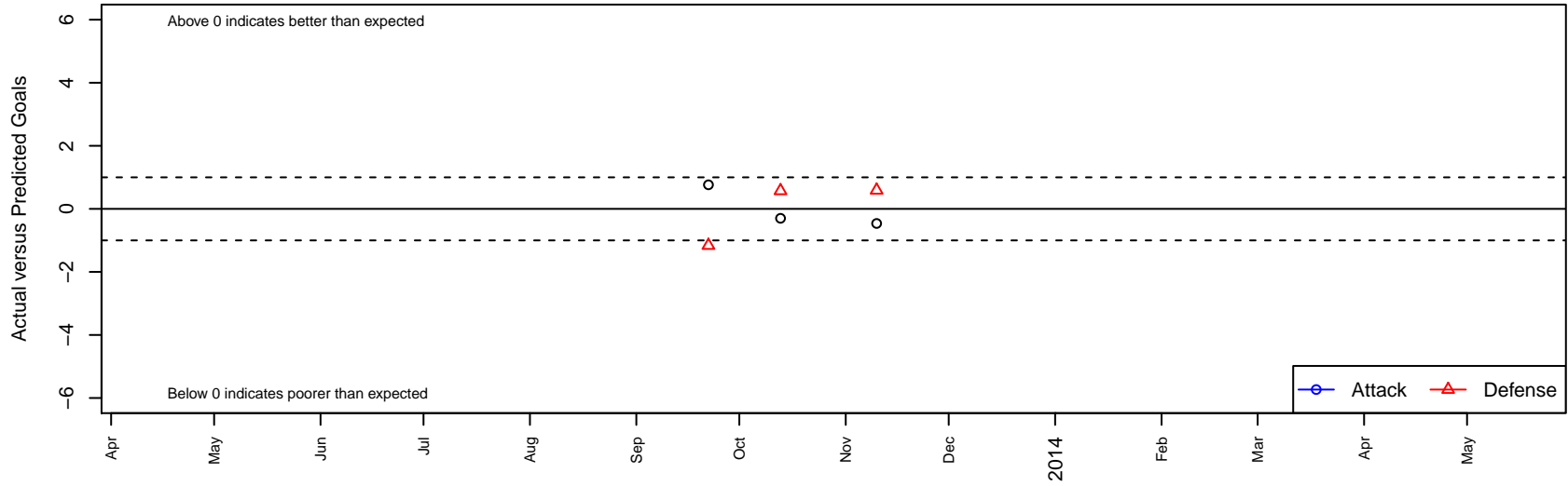
Impact SC B99 Dots are actual minus expected GF (blue circles) and GA (red triangles). Blue line is smoothed change in attack strength. Red is smoothed change in defense strength.
